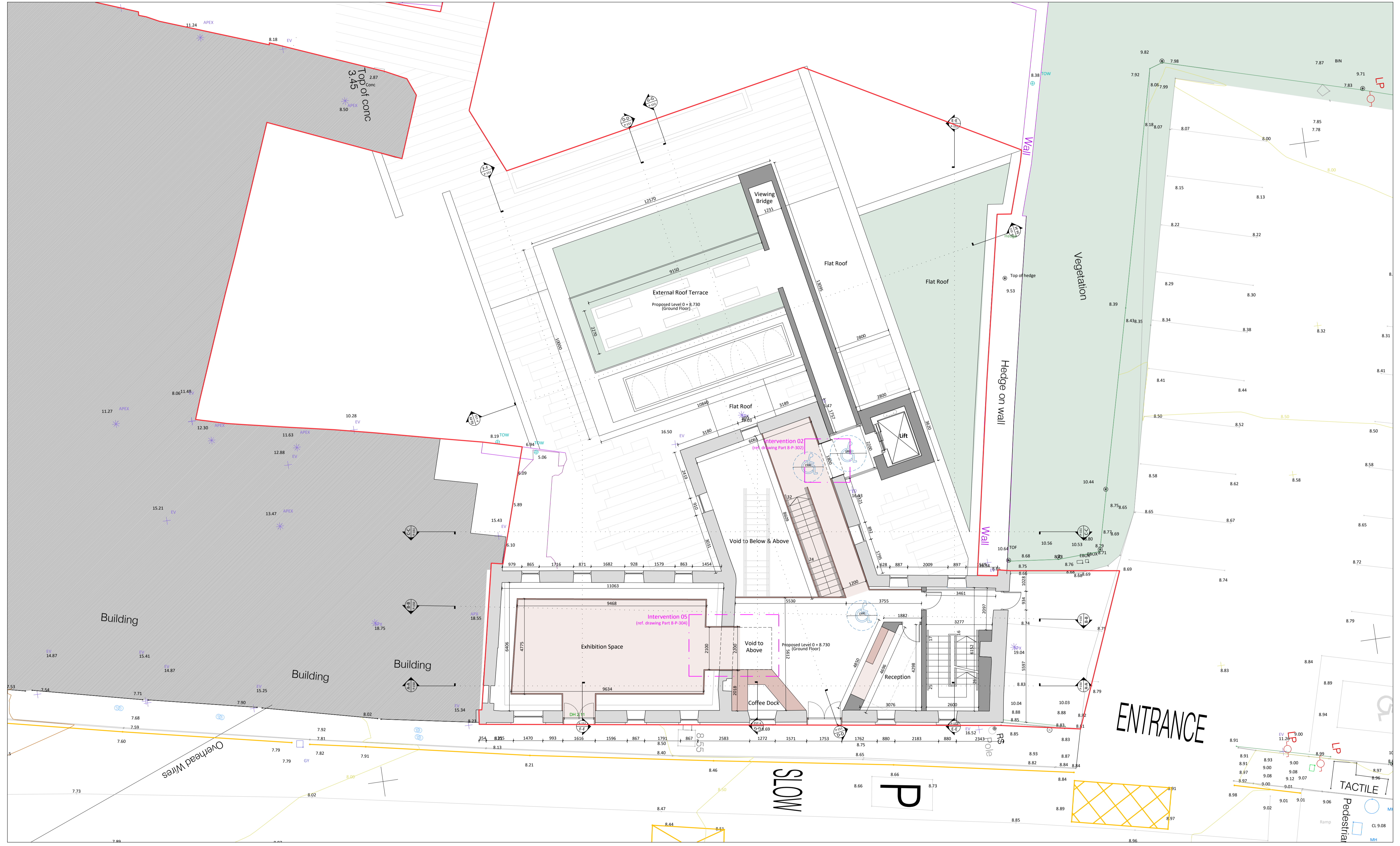
01 Level 0 (John Street) Floor Plan As Proposed Scale: 1:100
